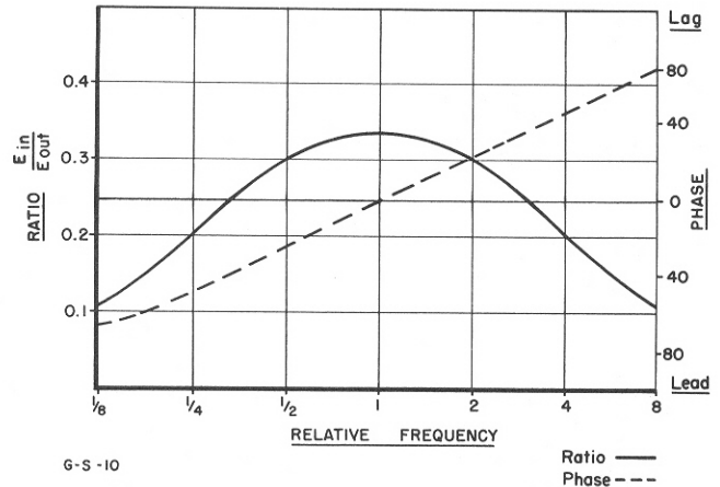
Figure 4-3. Oscillator Network Characteristics
