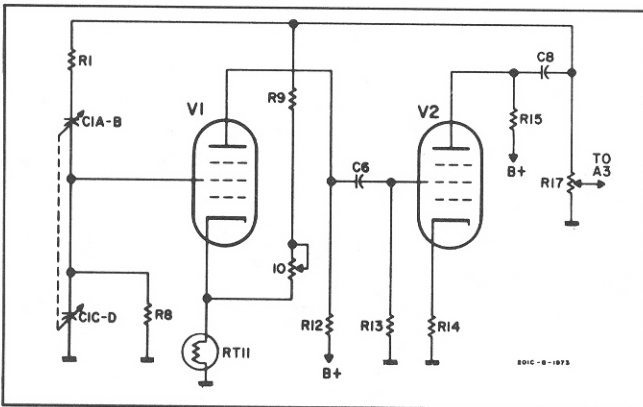
Figure 4-2. Simplified Schematic Diagram of Oscillator Section
