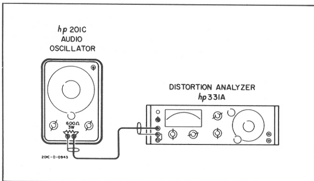
Figure 5-3. Distortion Check
